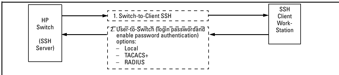
Figure 4-2. Switch/User Authentication
