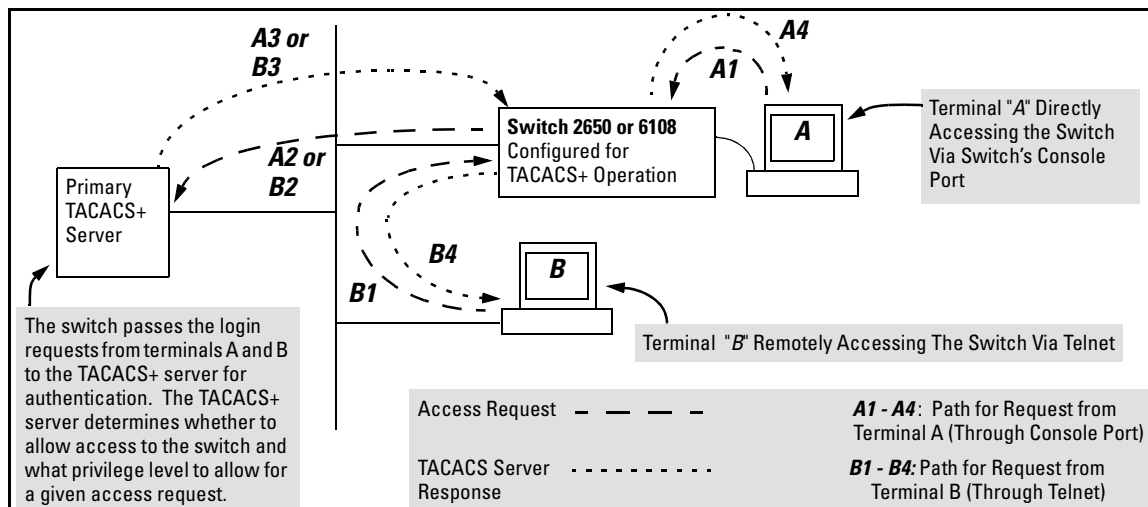
Figure 2-1. Example of TACACS+ Operation
