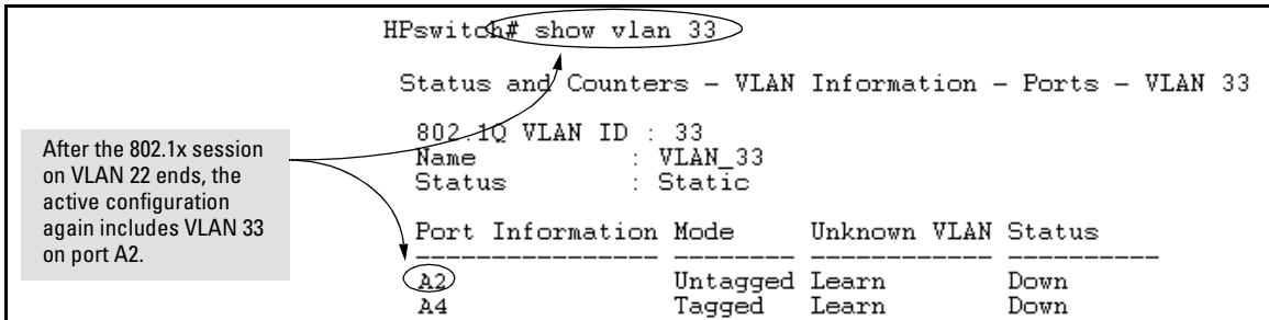
Figure 5-8. The Active Configuration for VLAN 33 Restores Port A2 After the 802.1x Session Ends
