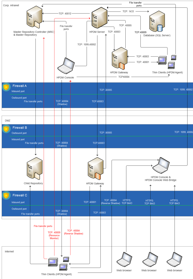
Figure 5. Typical HPDM topology in a DMZ environment
