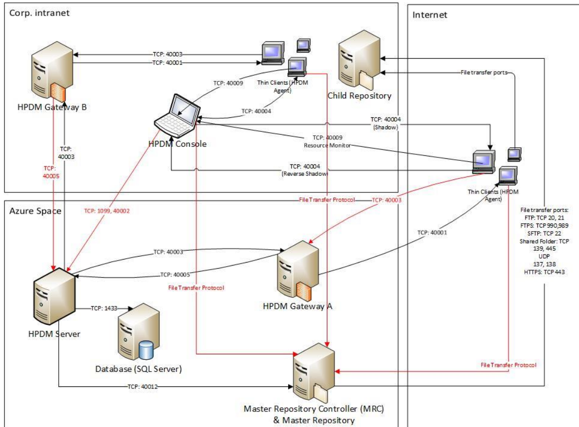
Figure 7. Typical topography
